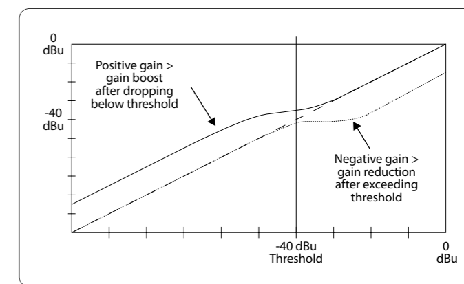
Fig. 4.36: Filter curves with gain above/below threshold
