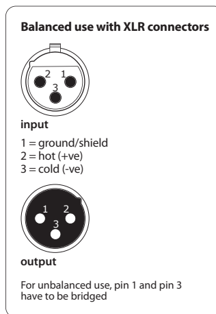
Fig. 4.2: XLR connections
