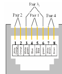
T568B Line sequence
